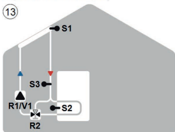
Solar com bypass
